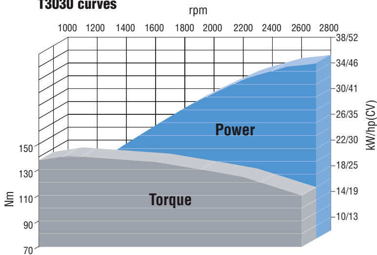
T3030 curves
