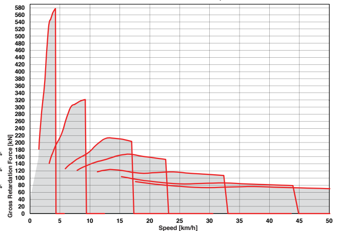
ADT, B60E 4X4 - Retardation
