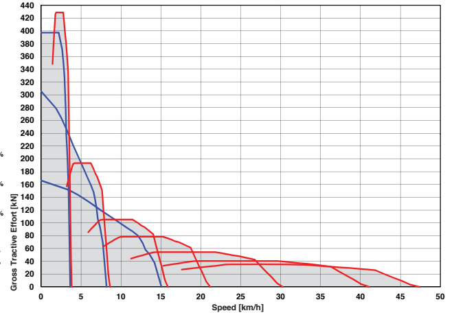
ADT, B60E 4X4 - Tractive Effort
